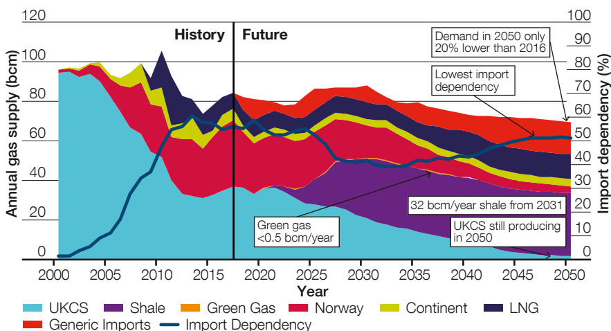
Figure 4.16 Annual supply pattern in Consumer Power
