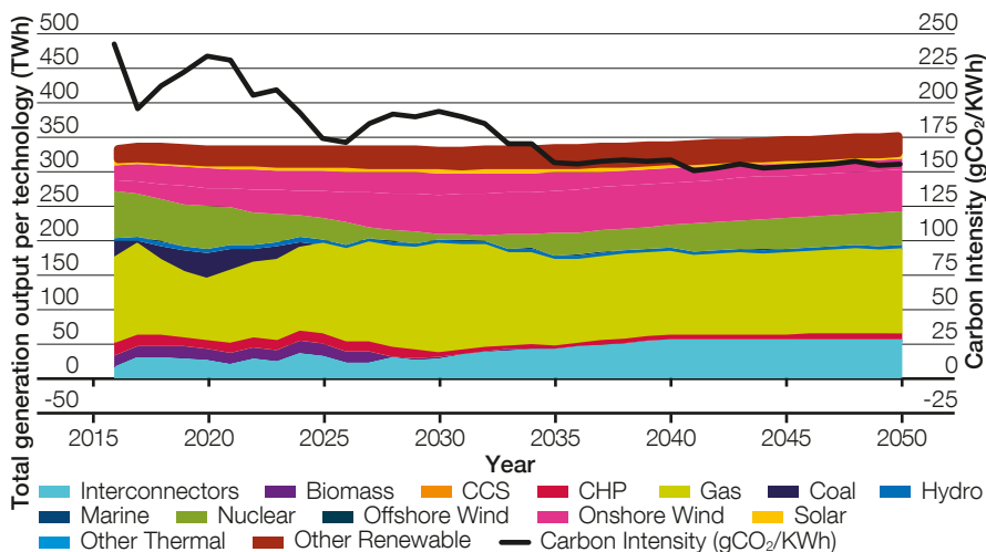
Figure 4.4 Generation output and carbon intensity – Steady State
