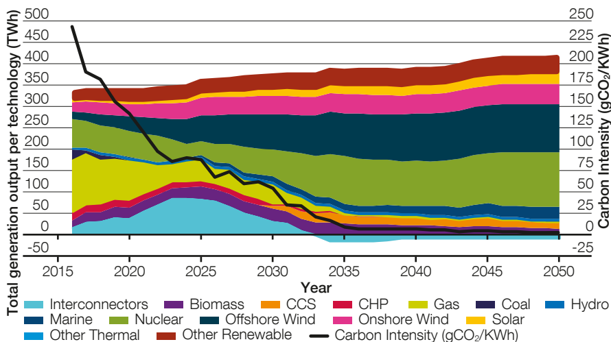
Figure 4.3 Generation output and carbon intensity – Two Degrees
